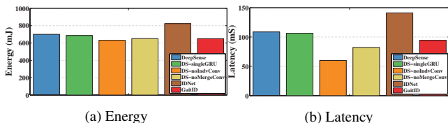
Figure 17: Energy and Latency of UserID solutions on Edison
