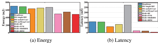
Figure 16: Energy and Latency of HHAR solutions on Edison
