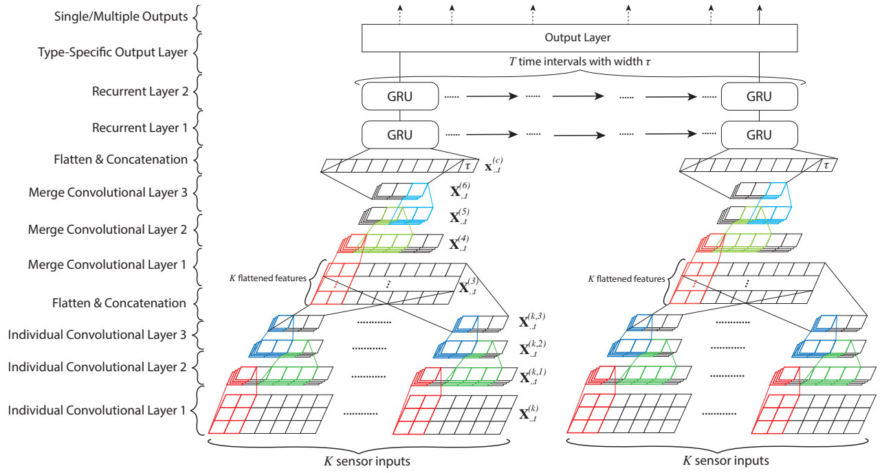
Figure 1: Main architecture of the DeepSense framework.
