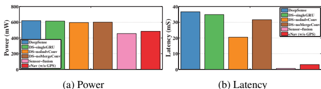
Figure 15: Power and Latency of carTrack solutions on Edison
